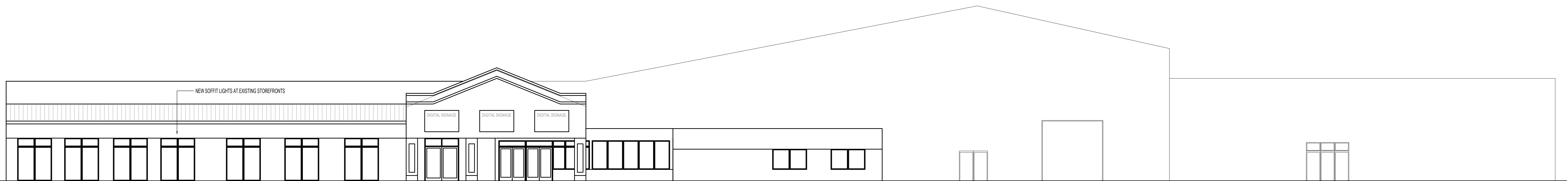
NORTH ENTRY HALL A ELEVATION 1/8" = 1'-0"
